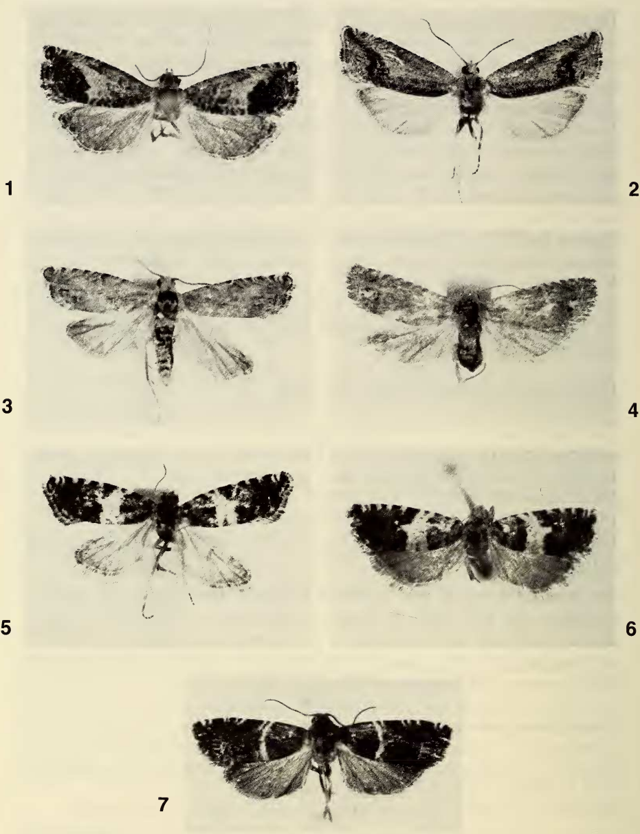
Figs 1-7. Adults of Grapholitini. 1 - Cydia johanssoni sp.n., holotype; 2 - Cydia blackmoreana (WALS.), male, Libya; 3 - Cydia tunisiana sp.n., male paratype; 4 - Lathronympha christenseni sp.n., holotype; 5 - Cydia ? plumbiferana (STGR), male, Greece, Taiyeto Mts; 6 - Cydia plumbiferana (STGR), holotype; 7 - Cydia alienana (CAR.), male, Turkey, Mersin.
